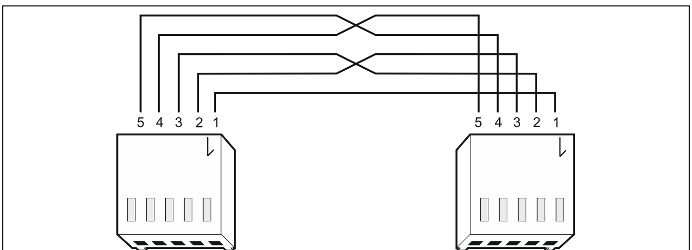
Fig. 3. Wiring diagram of the cable connecting RS-232 ports of ETHM-1 Plus module and INTEGRA control panel with PIN5 connector socket.
