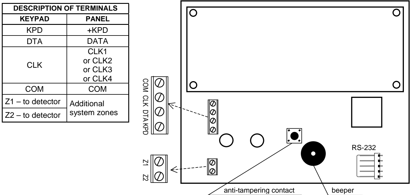
Figure 2. Schematic view of the keypad board including designations of wire terminals (version LCD-L V1.2).
